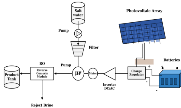
Figure 4 Schematic diagram of a PV-powered reverse-osmosis system. Reproduced from (Tigrine et al., 2016).
