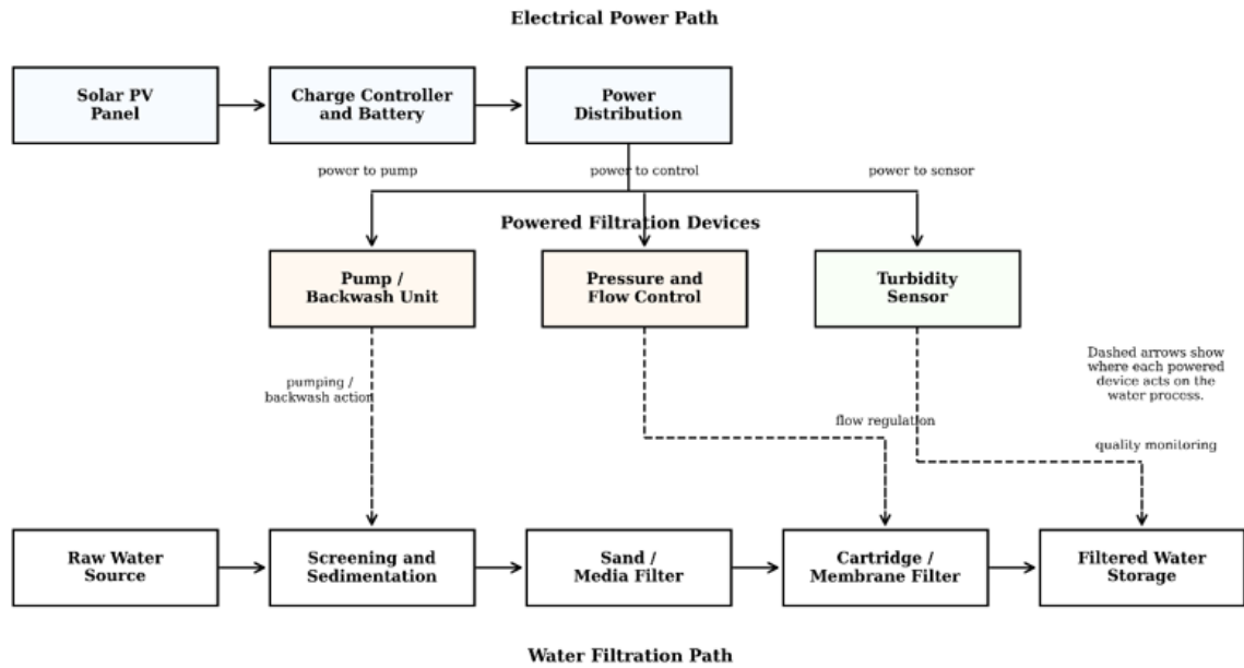
Figure 6 Schematic pathway for PV-powered filtration. Source: Authors' original illustration based on the working principles described in the text.
