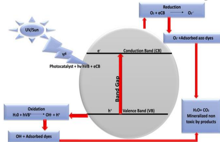
Figure 8 Mechanism of azo-dye degradation in photocatalysis. Adapted from (Oyetade et al., 2022).
