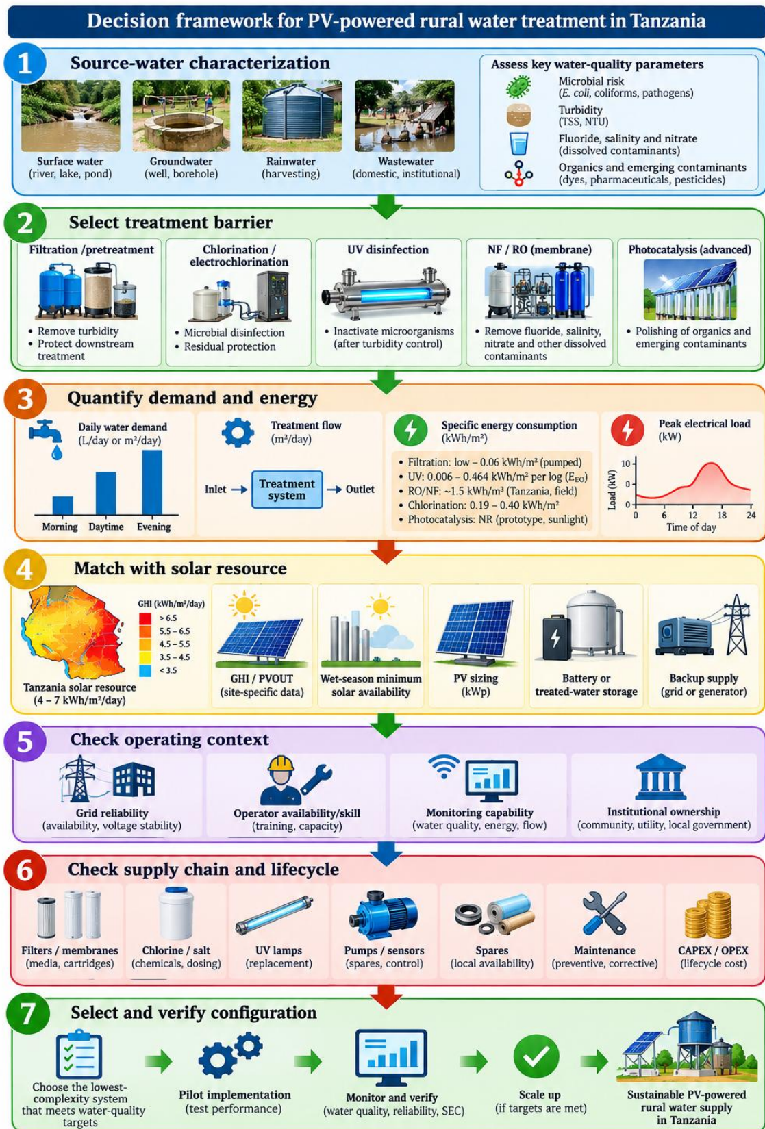
Figure 9 Decision framework for selecting PV-powered water-treatment configurations for rural Tanzania. Source: Authors' original synthesis based on the reviewed evidence.
