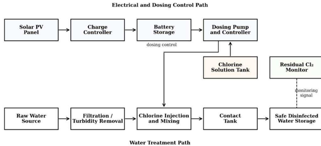
Figure 5 Schematic PV-powered chlorination pathway. Source: Authors' original illustration based on the working principles described in the text.
