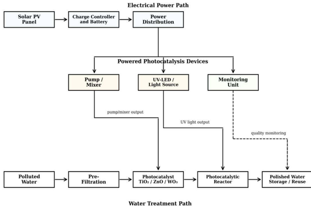
Figure 7 Schematic pathway for PV-powered photocatalysis. Source: Authors' original illustration based on the working principles described in the text.
