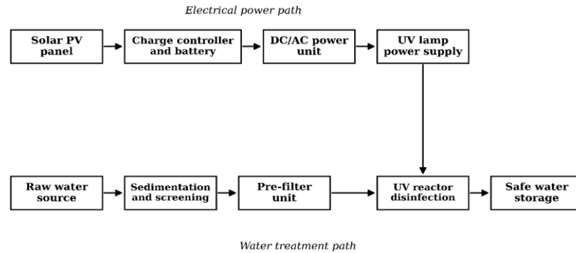
Figure 3 Schematic pathway for PV-powered UV disinfection. Source: Authors' original illustration based on the working principles described in the text.
