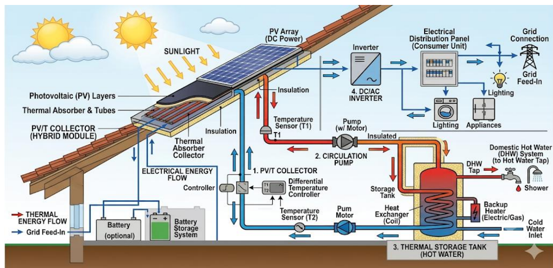
Figure 1: Schematic of PV-assisted solar thermal system (Herrando et al., 2023)
