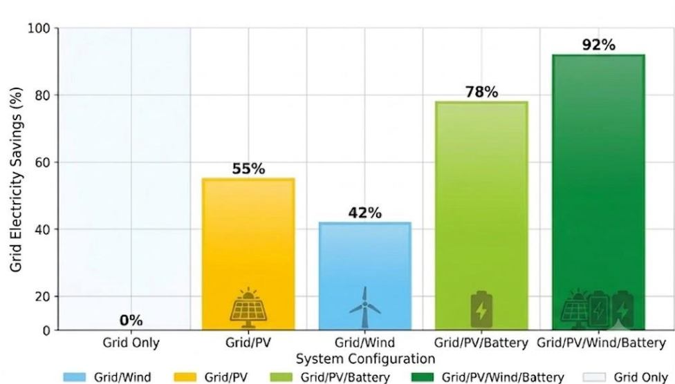
Figure 5: Grid Electricity Savings (%) Across Hybrid Configurations in Hotels(Serat et al., 2024)(Schleifer et al., 2023)
