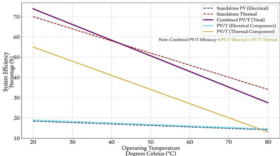
Figure 6: Graph of combined PV/T efficiency vs. standalone PV or thermal systems
