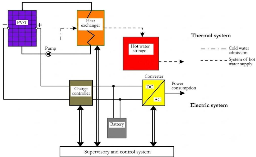
Figure 2: Diagram of PV/T collector showing electricity and heat generation (Herrando et al., 2023)
