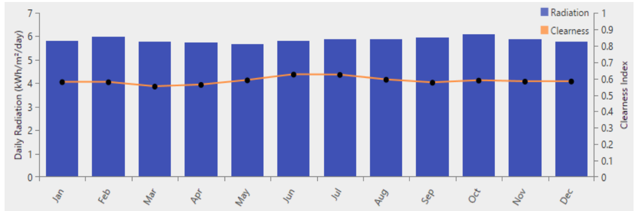
Figure 3 Monthly solar radiation given by HOMER software.
