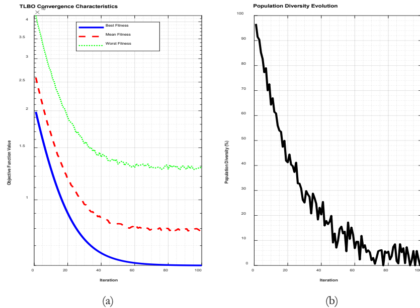
Figure 6 (a) TLBO Convergence Characteristics, (b) Population Diversity Evolution for the IEEE 14-bus system
