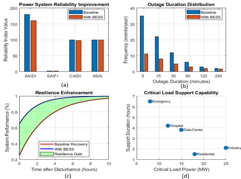
Figure 13 (a) The impact of BESS on system reliability, (b) the outage distribution frequency against the duration of the outage, (c) resilience gain on the IEEE 30-bus system and (d) the critical load support capability.
