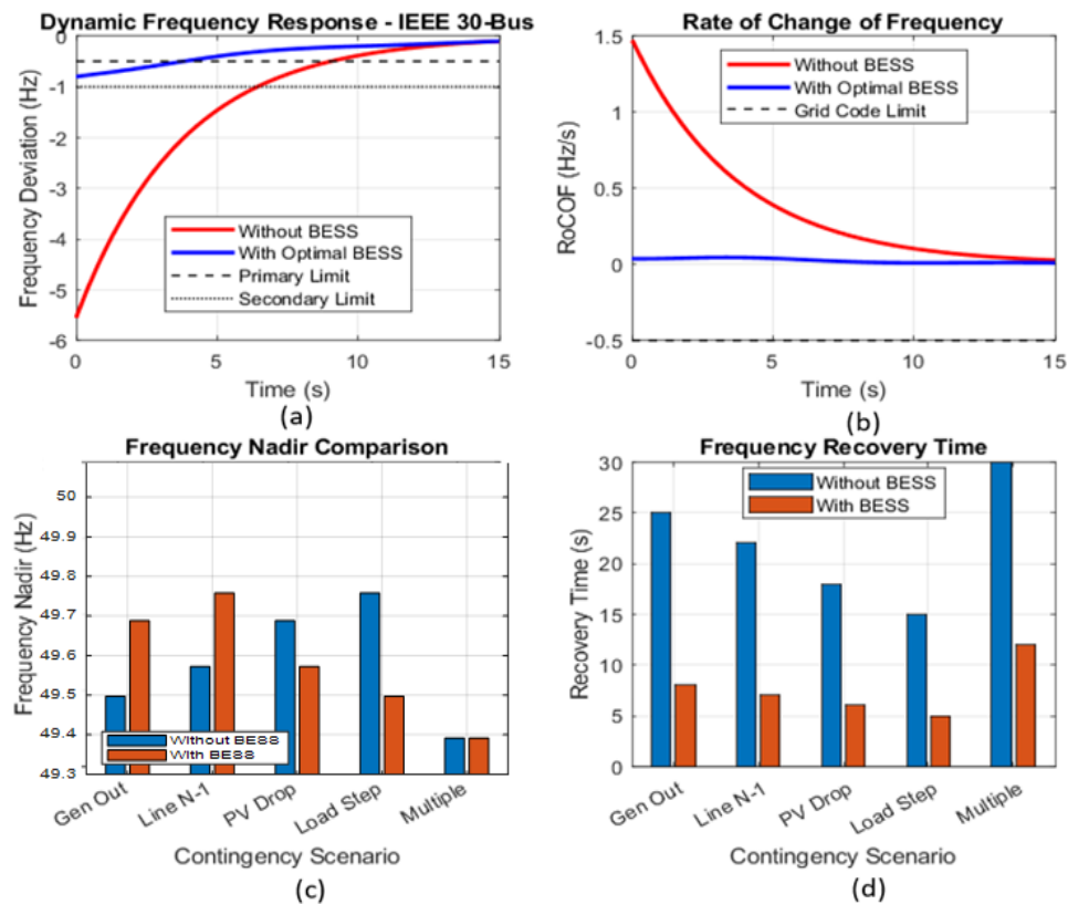
Figure 12 (a) The dynamic frequency response in the IEEE 30-bus system, (b) the rate of change of frequency, (c) The comparison of Nadir frequency at different contingency scenarios and (d) Frequency recovery at different contingency scenarios.
